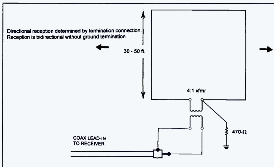
Mediumwave version of K9AY terminated loop antenna.
