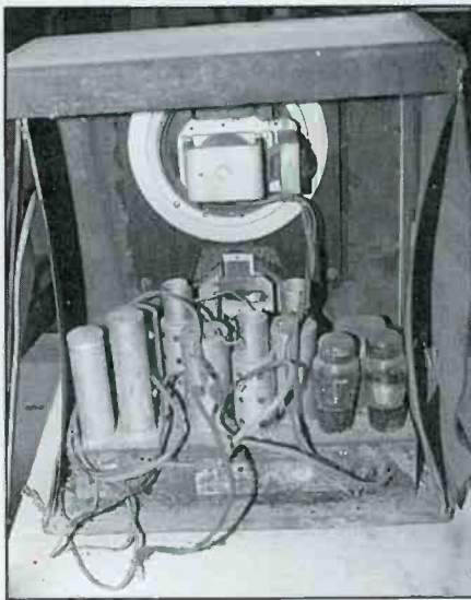
The rear view tells all. The sides are completely destroyed from decades of moisture. The chassis is coated with dirt, and the chassis side aprons are rusted through.
