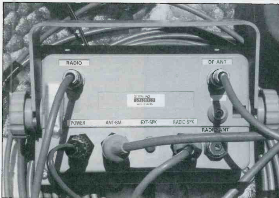
The rear panel on an ADF rig.
