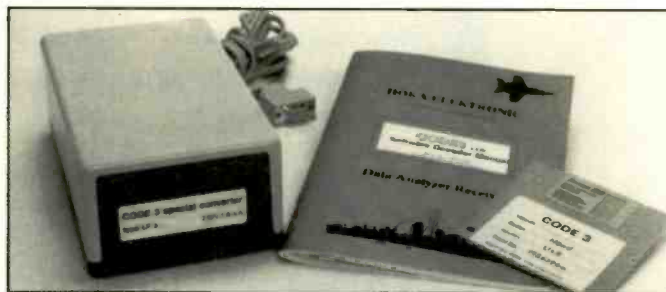
Hoka Code 3 is a multilevel system allowing the interfacing of a computer with a communications receiver to produce a number of benefits, including SITOR reception. It's from Computer Aided Technologies.
