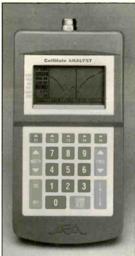
The CellMate from AEA checks out antennas operating in the 806-960 MHz range.
