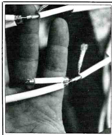
Close-up of phasing harness that goes inside the fiberglass mast.
