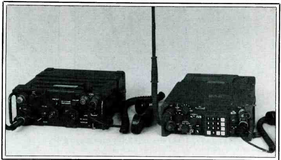
SINCGARS demonstrates the revolutionary improvements in performance provided by microelectronics adapted to the battlefield. Shown here at left is the Vietnam-era AN/PRC-77 manpack (still used by the Marine Corps), which communicates over 920 channels, but now achieves only about 100 hours mean time between failures (MTBF). The smaller and lighter SINCGARS PRC-119 at right will make 2,320 channels available to user units. SINCGARS field tests have produced MTBFs in excess of 5,000 hours.
