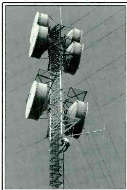
Army MARS member Ed Kaleta (AAT5IA) installs a 49.79 MHz link antenna on an M.C.I. tower in Petersburg, Michigan. An Army MARS 143.99 MHz repeater antenna is at the top of this tower. (Photo by John S. Papay, K8YSE/AAR5WI)
