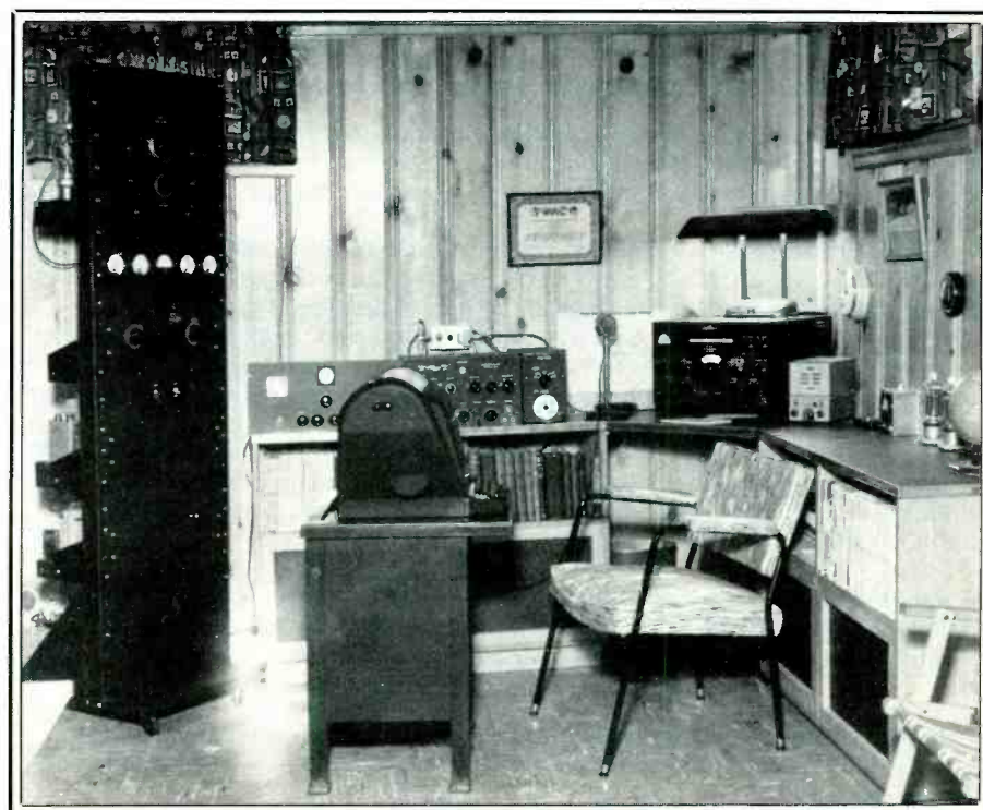
An old-style RTTY station using the bulky equipment that has mostly been replaced by modern technology. This stuff clattered away and sounded like a Thompson submachine gun!
