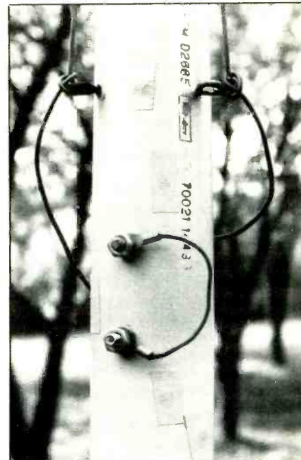
Figure 3: Easy-reach position of jumper.
