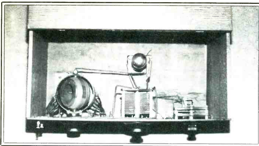
A look inside, lid open showing variocoupler two condensers and tube.
