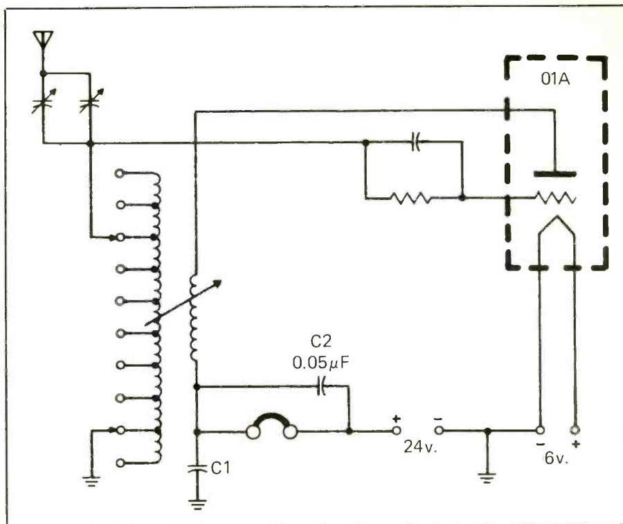
Figure 2: Antique radio circuit as modified.
