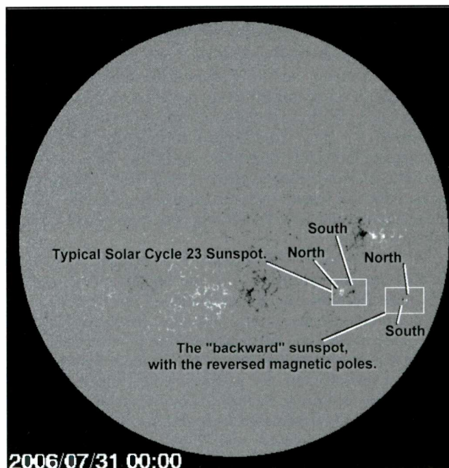
A view of the sun that reveals the magnetic orientation of several sunspots occurring on July 31, 2006. The darker areas indicate a south magnetic "pole," while the lighter areas indicate a north magnetic "pole." The sunspot that has a backward-oriented polarity is the likely signal that a new solar cycle is starting. (Source: NASA/SOHO)
