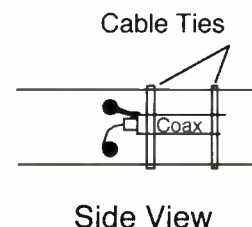
Figure 2. Fifty- and 72-ohm element spacing.
