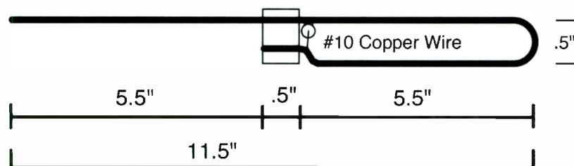
Figure 1. Driven element dimensions.
