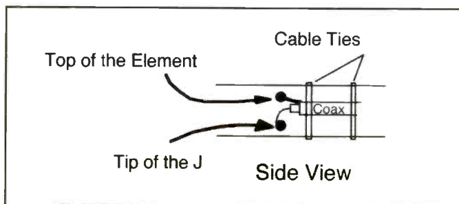
Figure 3. Coax attachment.
