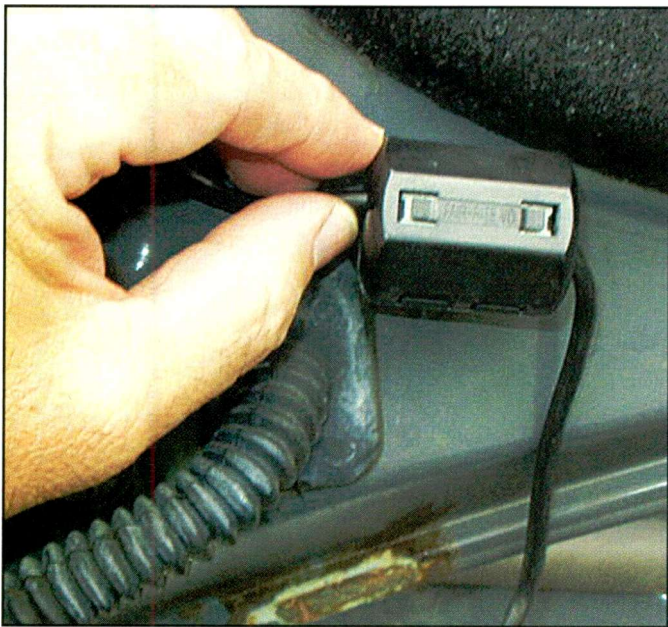
The ferrite core must be placed on the control cable to keep antenna motor noise down during tuning. It also decouples the control wire from antenna.
