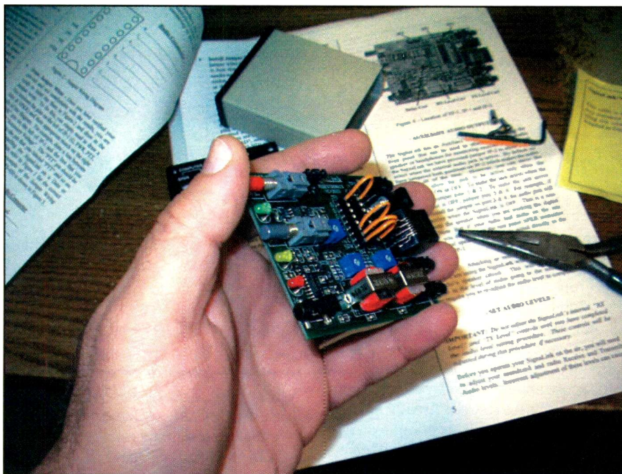
Here's an inside look at the Signalink SL-1+ unit. The jumper wires have been carefully inserted with small needle-nose pliers.
