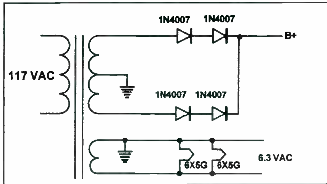
Figure 2. The 6X5 rectifiers can be replaced by two sets of 1N4007 diodes mounted on terminal strips. All leads to the 6X5 cathode and plate pins must be removed and rerouted. Only the filament connections remain. The 6X5 filaments provide the nostalgia, while the silicon diodes do the work.
