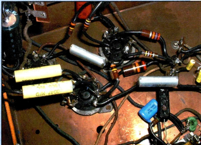
Photo B. Desoldering the old parts is a lot of labor, it but keeps things neat under chassis. Be careful not to damage the tube socket terminals or other tie points when removing the old leads. I also advocate using PVC jacketed fiberglass spaghetti over the component leads.
