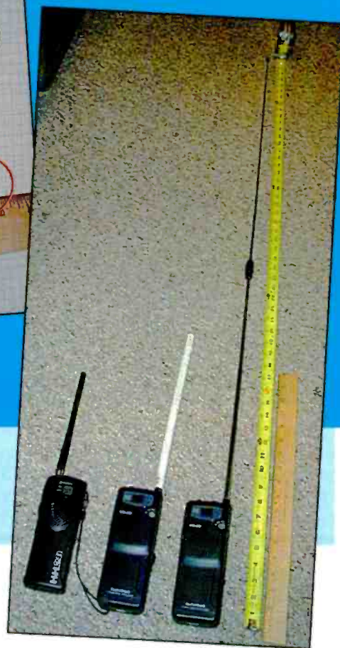
CB with semi-flex antenna, CB with rubber ducky, and normal CB antenna out. →
