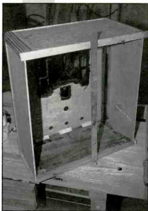
Photo 10. Constant rechecking, and using a square will ensure everything will fit as intended when the final glue-up takes place.
