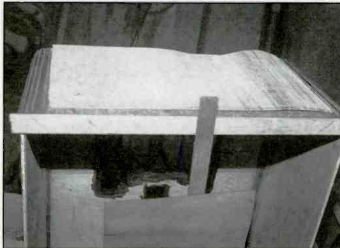
Photo 9. The top veneer core is also used as a template when cutting the new top panel.
