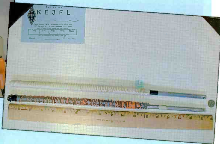
The finished antenna with and without heat shrink tubing cover.
